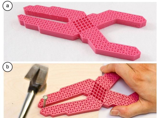
Figure 10: (a) This pair of pliers is based on a single metamaterial four-bar. (b) When the user applies a force to the handles, the hinge array in the center transmits this force to the brackets, and the pliers close.
