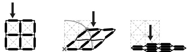
Figure 12: When a shear cell in this 2 \times 2 block is subject to compression forces, it complies by shearing on a circular trajectory until its members are packed tightly.
